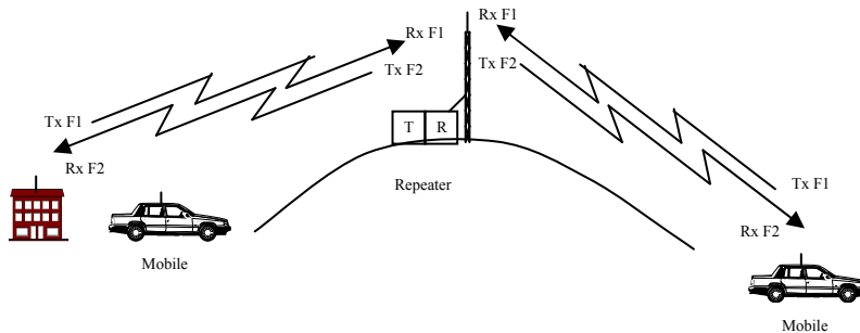
Figure 1: Conventional Repeater System
